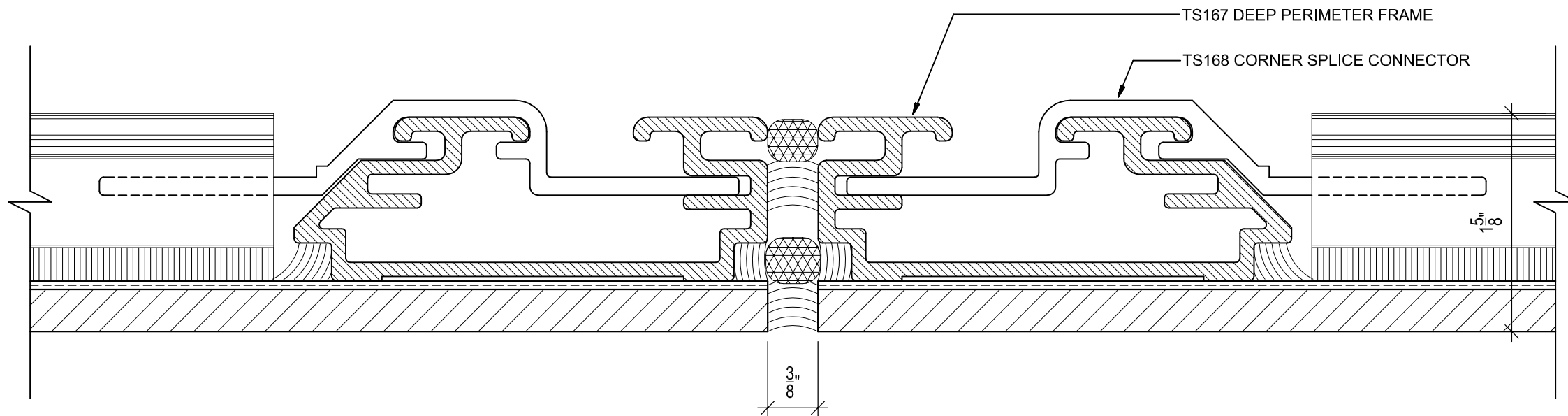
TS167 DEEP PERIMETER FRAME SCALE: FULL-SIZE
