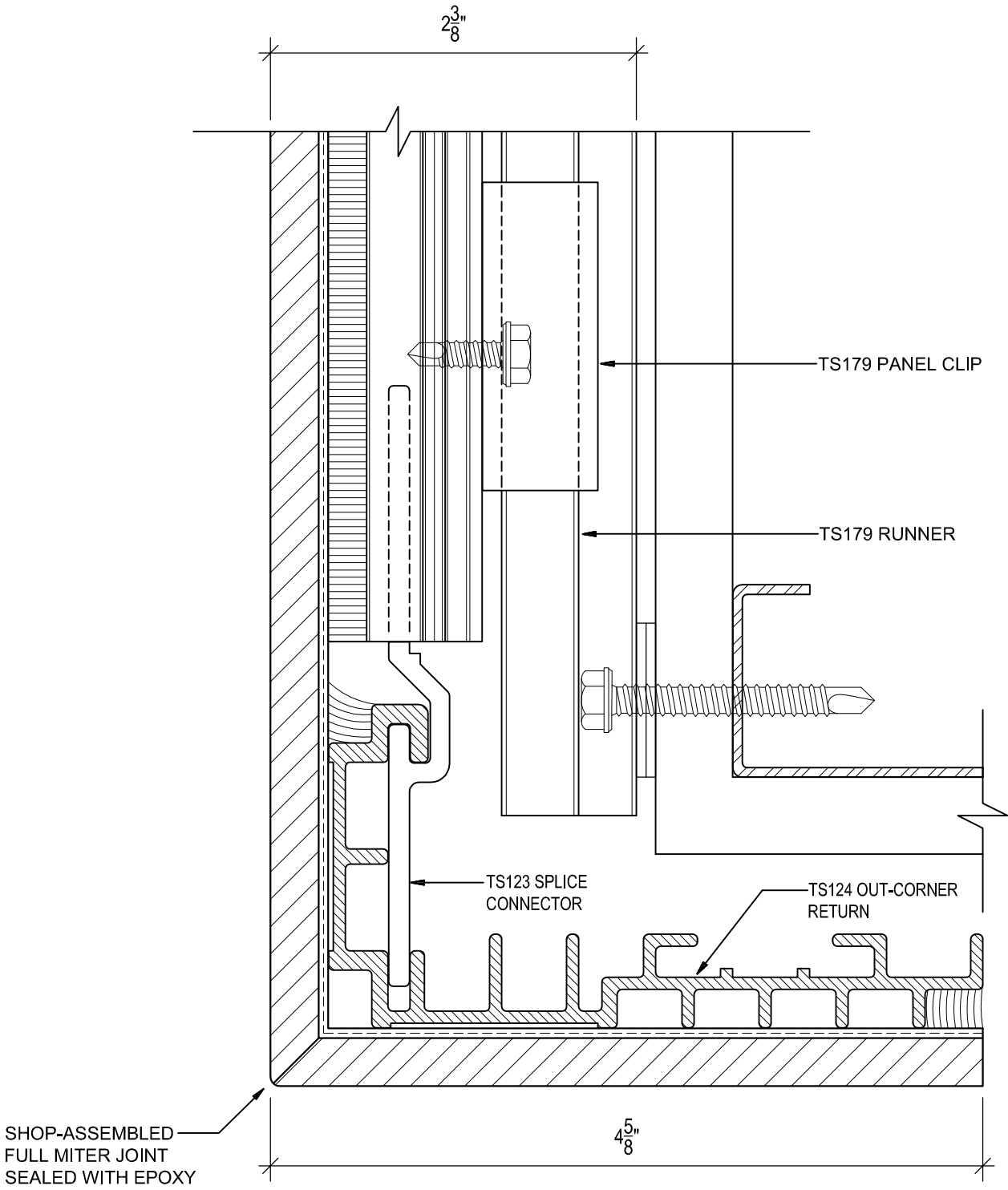
TS124 OUT-CORNER WITH 4 3/8" RETURN SCALE: FULL-SIZE
