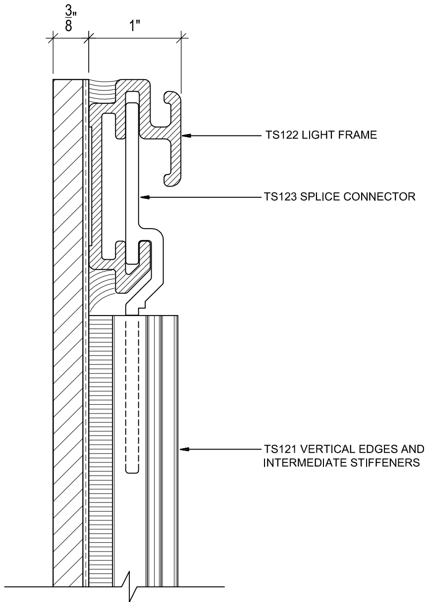
TS122 - LIGHT FRAME SCALE: FULL-SIZE
